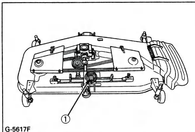
(1) Grease nipple (Balance shaft)
