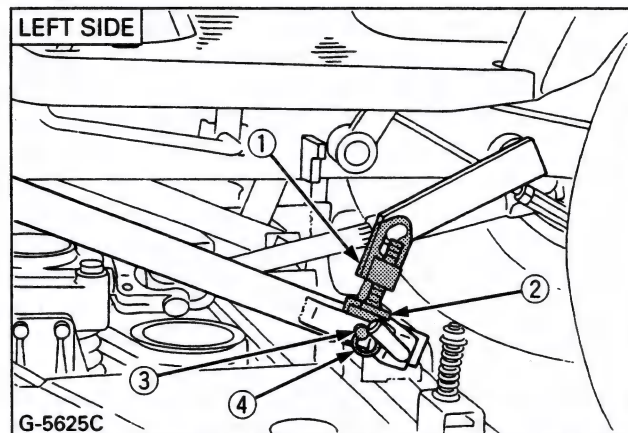
(1) Lift link (Upper)
