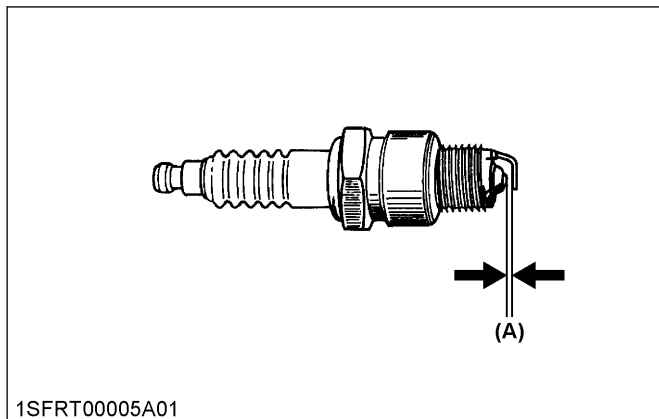
(A) 0.7 to 0.8 mm, 0.028 to 0.031 in.
