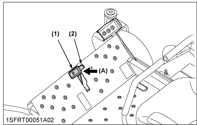
(1) Parking brake pedal (2) Parking brake lock pedal
