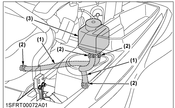
(1) Hydraulic hose (2) Hose clamp
