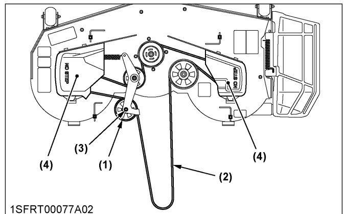
(1) Tension pulley
