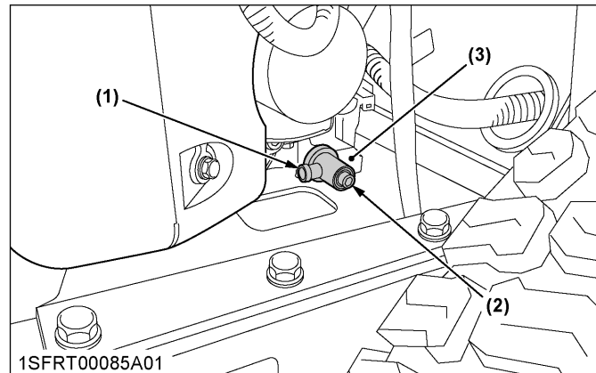
(1) Oil drain valve (2) Hex plug
